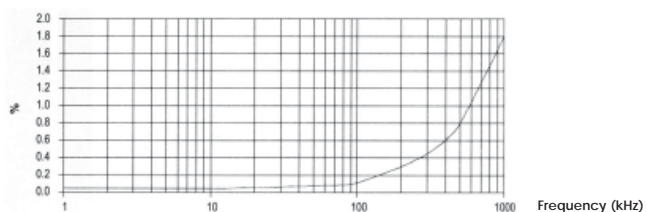
Figure 4: Distortion (Typical) Distortion measurements were made operating the amplifier at 75 % of the maximum Vpp output obtained from Figure 3.
